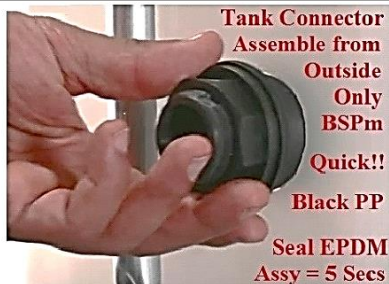
Extended fitting - Push into tank Wall Hole From Outside
