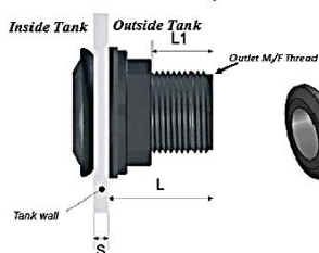
Mounted fitting - Screwed up from Outside - Easy
