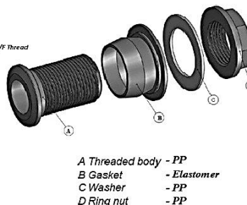
Fitting exploded view -
